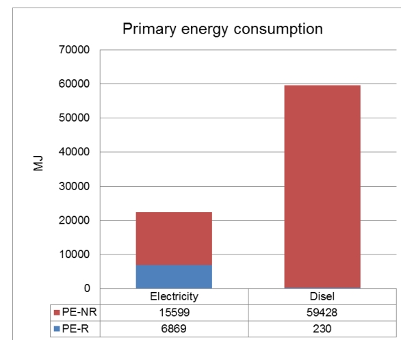
Figure 6.3-10: Primary energy consumption during on-site construction process of Joensuun Elli (wooden building elements only) according to the consumed energy resources
