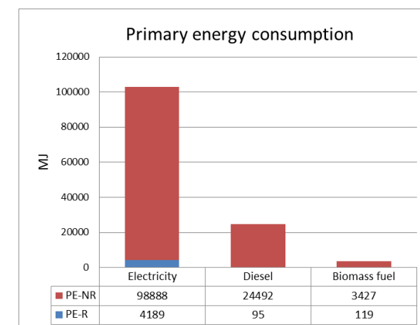
Figure 6.3-4: Primary energy consumption during the prefabrication process of Mietraching (wooden building elements only) according to the consumed energy resources
