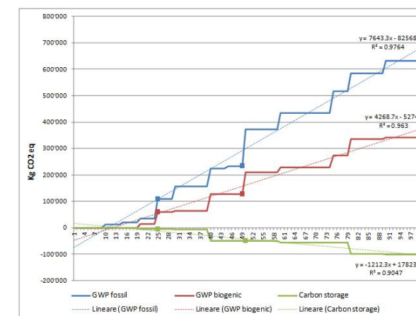
Figure 6.4- 9: GHG fossil and biogenic emission and carbon storage over the time for maintenance (module B2) and replacement (B4) activities, L'Aquila building. The RSL of products were assumed from BLP Durability Assessment report [7] considering the k-factorial method for the prediction of the ESLs.
