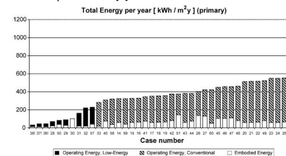
Figure 6.4-4: Primary energy consumption per m 2 of living area for different analyzed case studies. [2]
