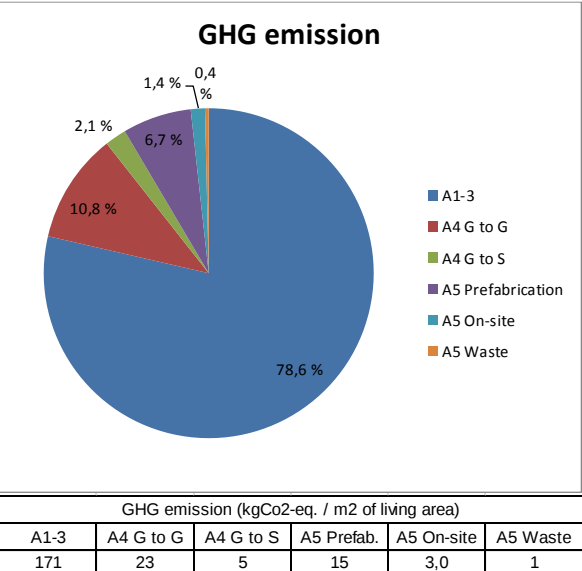
Figure 6.3-1: GHG emission during the production stage of Mietraching
