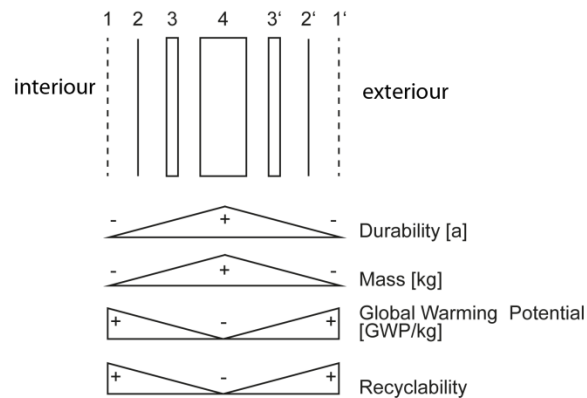
Figure 6.5-2: Sequence of technical and functional layers and weighted influence on EoL impact below. [8]
