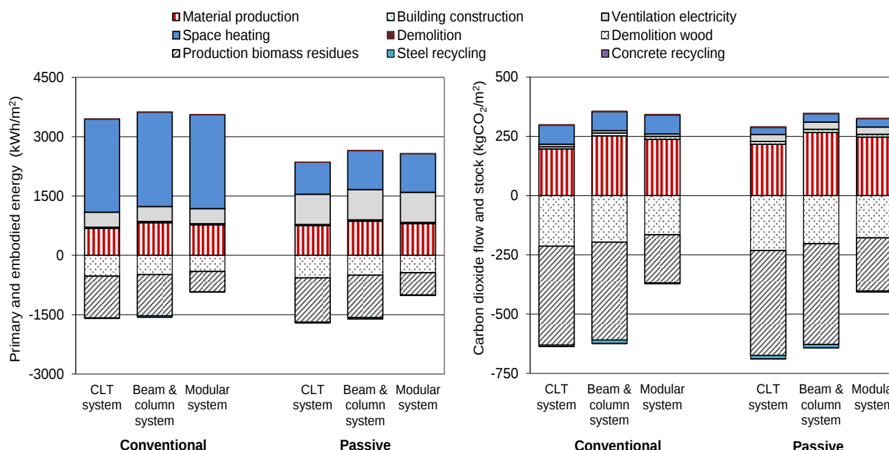
Figure 8.2-5: Primary energy use (a) and GHG emission (b) for the life cycle phases of the district heated buildings with assumed lifespan of 50 years. Energysupply is based on BST technology. Positive numbers denote energy use or GHG emission to the atmosphere. Negative numbers denote lower heating value of recovered biomass residues or GHG emission avoided if fossil coal is replaced.
