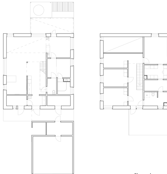
Floor plans
