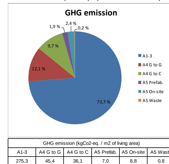
Figure 6.3-3: GHG emission during the production stage of Joensuu Elli
