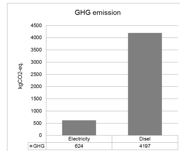
Figure 6.3-9: GHG emission from different energy source during on-site construction work of Joensuun Elli (wooden building elements only)
