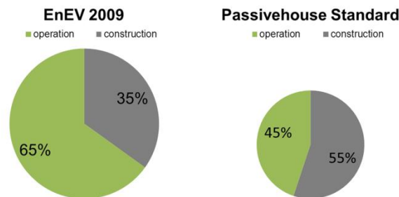
Figure 6.1-1: Dominance of construction and operation of different energetic standards in a life cycle analysis of an exemplary comparison [1]
