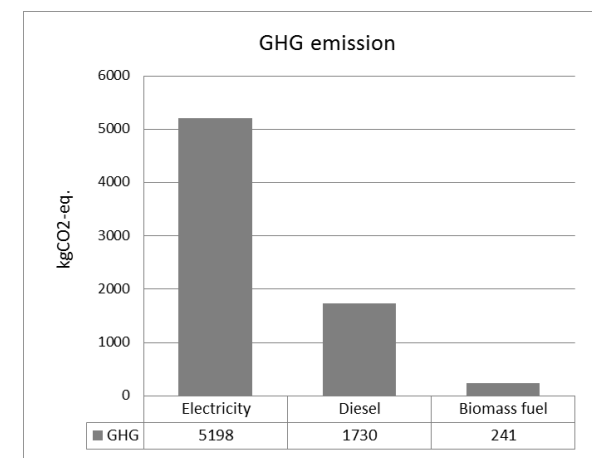
Figure 6.3-5: GHG emission from different energy source during prefabrication of Mitraching (wooden building elements only)
