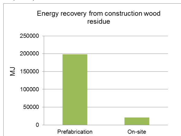
Figure 6.3-12: Tentative comparison of energy recovery capacity from wood residues generated from the two different construction systems in Mietraching
