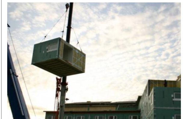
Figure 8.2-4: Volumetric modular system
