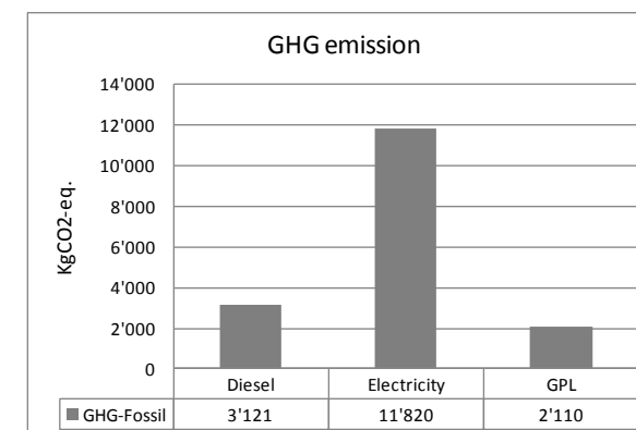
Figure 6.3-7: GHG emission from different energy source during on-site construction work of L'Aquila (wooden building elements only)
