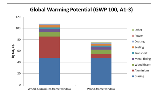
Figure 5.4-2: Carbon footprint of different phases of the windows manufacturing.
