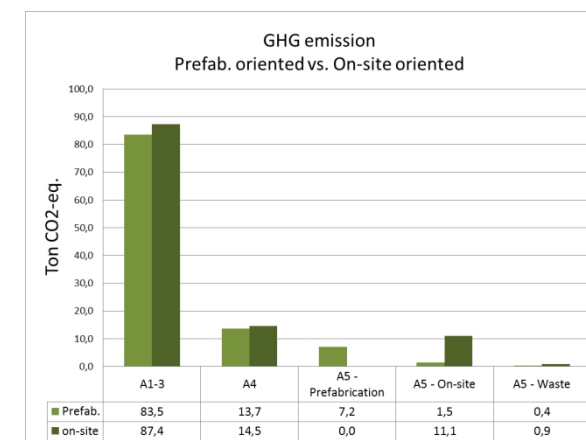
Figure 6.3-12: Tentative comparison of prefabrication oriented construction and on-site oriented construction regarding GHG emission during module A1-5 based on the Mietraching
