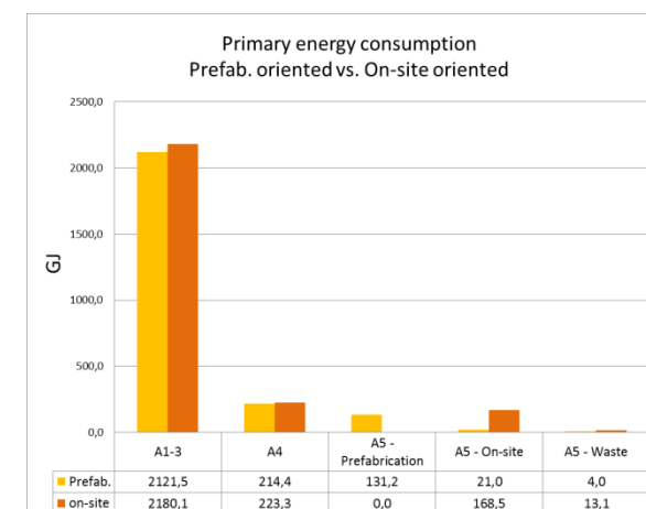
Figure 6.3-11: Tentative comparison of prefabrication oriented construction and on-site oriented construction regarding primary energy consumption during module A1-5 based on the case of Mietraching
