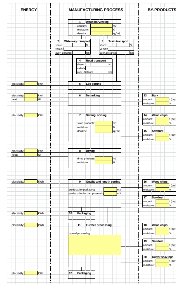
Figure 4.3-2: Manufacturing flow for the sawn timber.
