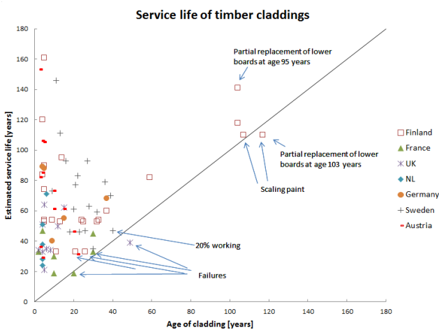
Figure 7.5-1: Comparison of the estimated service life of claddings which were surveyed in the Woodexter project in different European countries.
