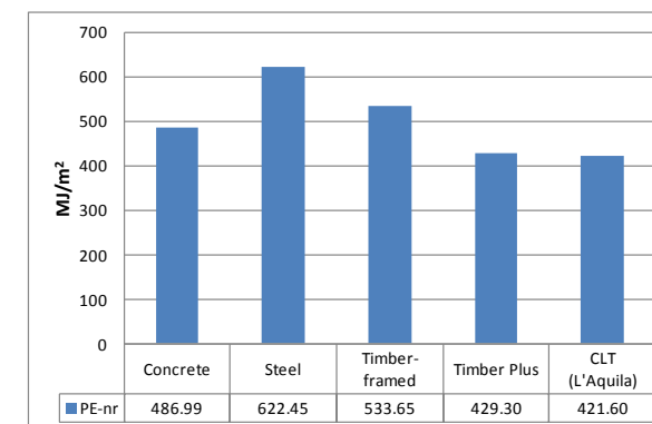
Figure 6.4- 7: Non-renewable primary energy consumption for maintenance. Three alternative material considered: concrete, steel and wood.
