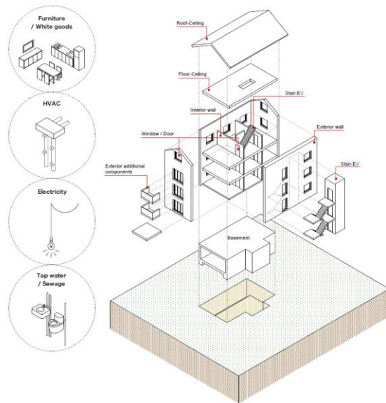
Figure 4.4-5: Example for visualization of included building elements
