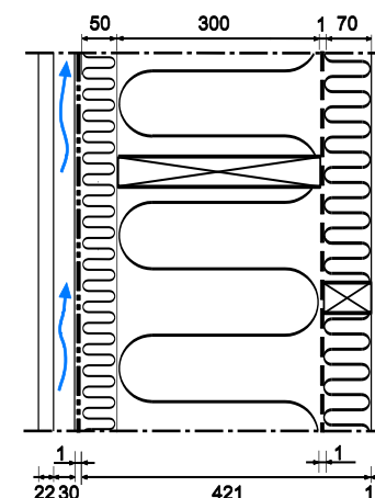
Figure 7.4-1: An example of wood framed external wall with a 30 mm well-ventilated air gap behind the cladding, 50 mm mould resistant insulation board protecting the organic studs and 70 mm insulated installation layer protecting the vapour barrier from installation works (Illustrator Lilian Johansson).
