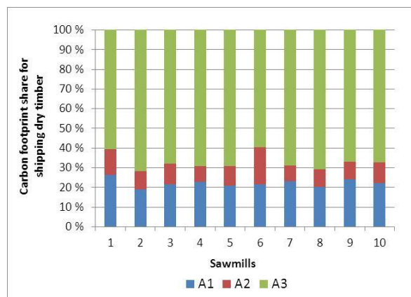
Figure 5.3-3: Carbon footprint and share of life cycle stages (A1, A2, A3) for shipping dry timber, Finland.
