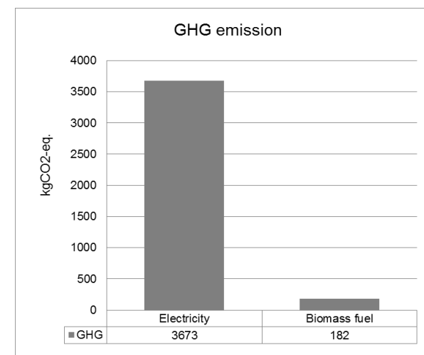
Figure 6.3-6: GHG emission from different energy source during prefabrication of Joensuu Elli (wooden building elements only)
