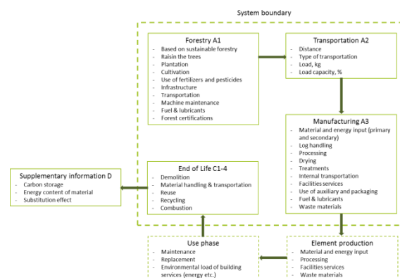
Figure 4.3-1: System boundary of wood based construction materials.
