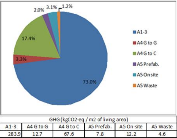
Figure 6.3-2: GHG emission during the production stage of L'Aquila
