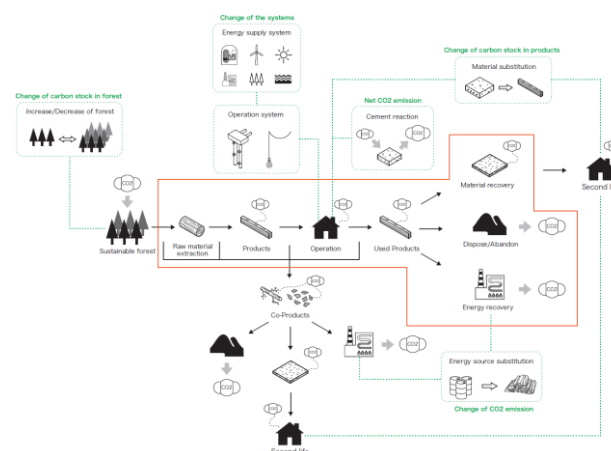
Figure 4.4-1: Holistic picture of carbon footprint related to a wood-based building system and simplified system boundary (red line) for the system building including only direct environmental effects.
