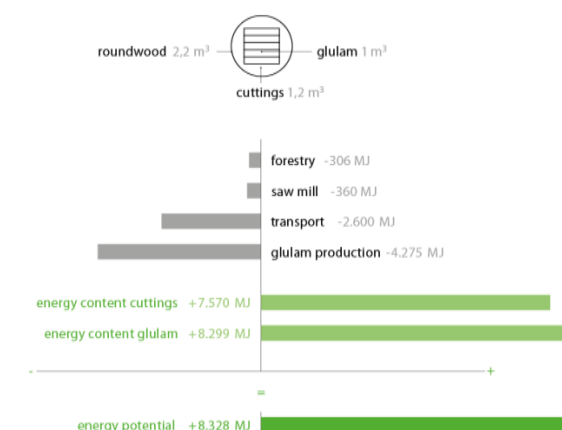
Figure 6.5-1: Material of 1 m³ of CLT stores biomass energy of 2313 kWh (8328 MJ) [2].
