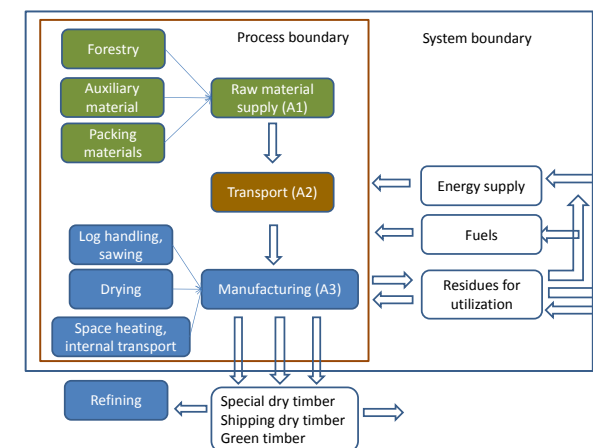
Figure 5.3-1: System boundary of studied system.
