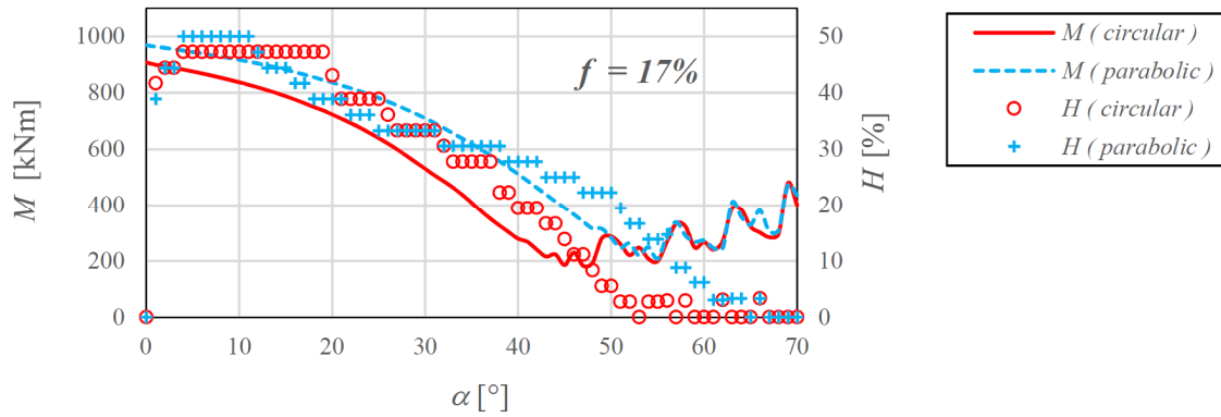
Figure 3.34 Maximum bending moment and percentage of relaxed hangers H as a function of angle \alpha in network radial pattern
