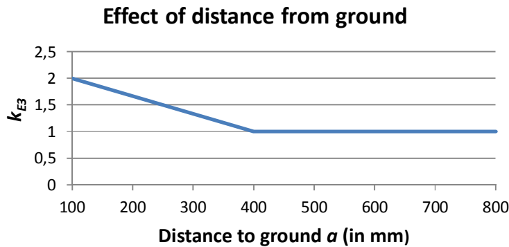
Figure 2.10. Effect of distance a from ground is described by the factor k_{E3} .
