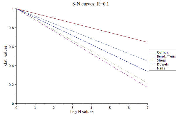
Figure 3.43 S - \log N curves for various stress types or connection types for R = 0.1
