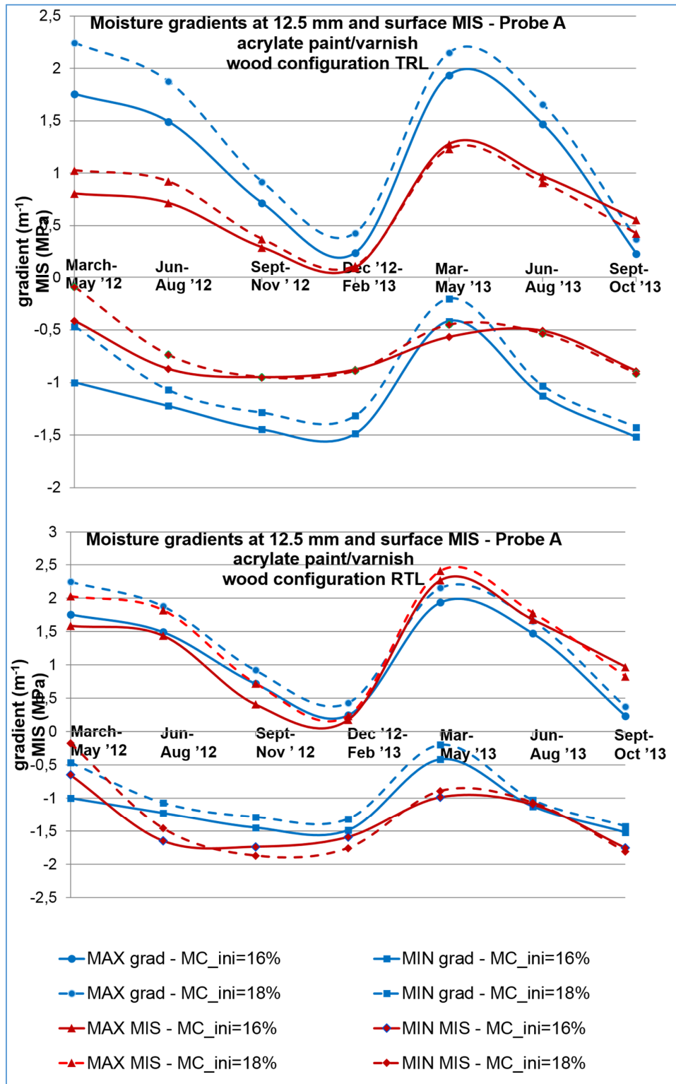
Figure 5.45. Probe A. Moisture gradients at 12.5 mm and surface MIS for different initial moisture contents ( MC_{ini} ) in the case of configuration TRL (top) and RTL (bottom).
