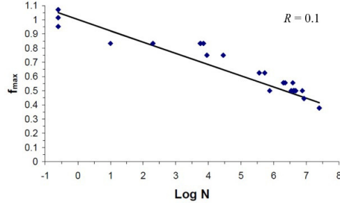
Figure 3.45 S - \log N curves for dowel connections obtained from tests with R = 0.1 (Malo, Holmestad et al. 2006)
