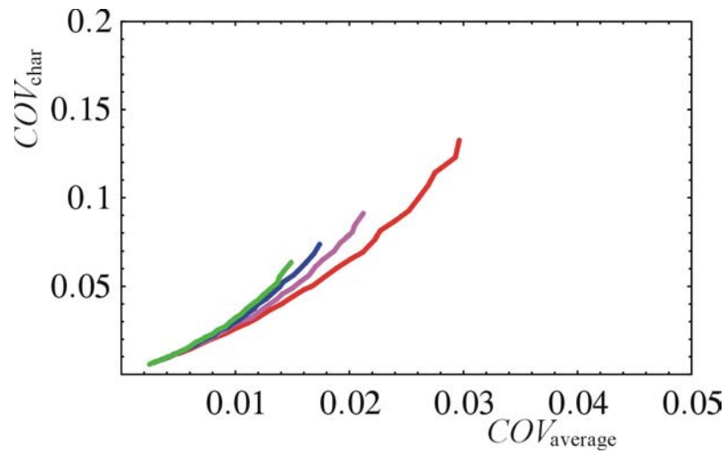
Figure A1. COV of characteristic value vs. COV of the average (COV of strength fixed).
