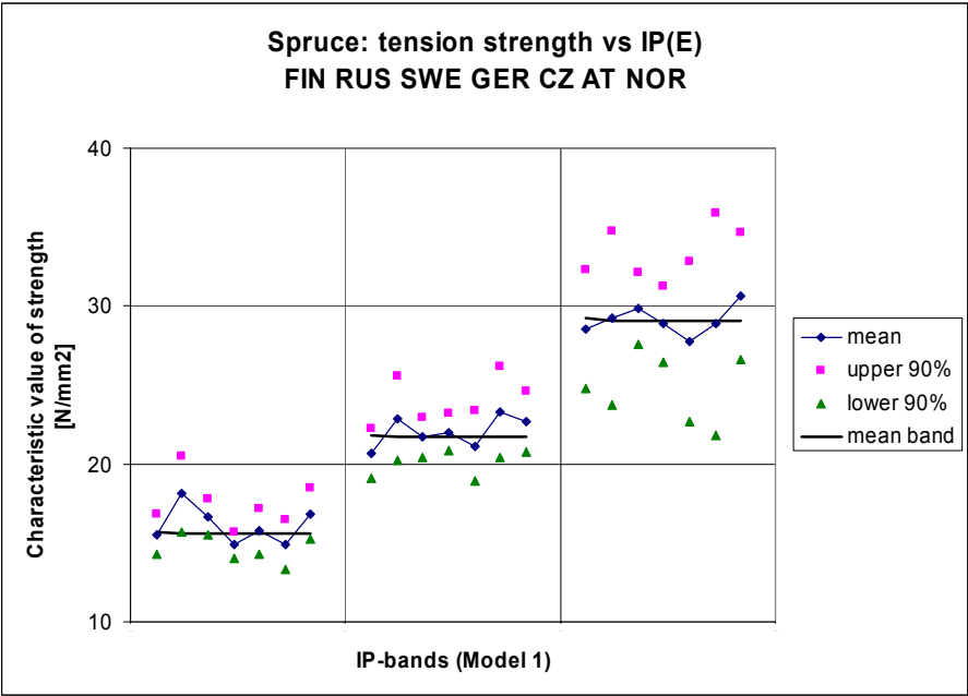
Figure 29. Comparison between countries, characteristic strength values with individual confidence limits. Spruce in tension, Model 1, based on same data as Fig. 28.
