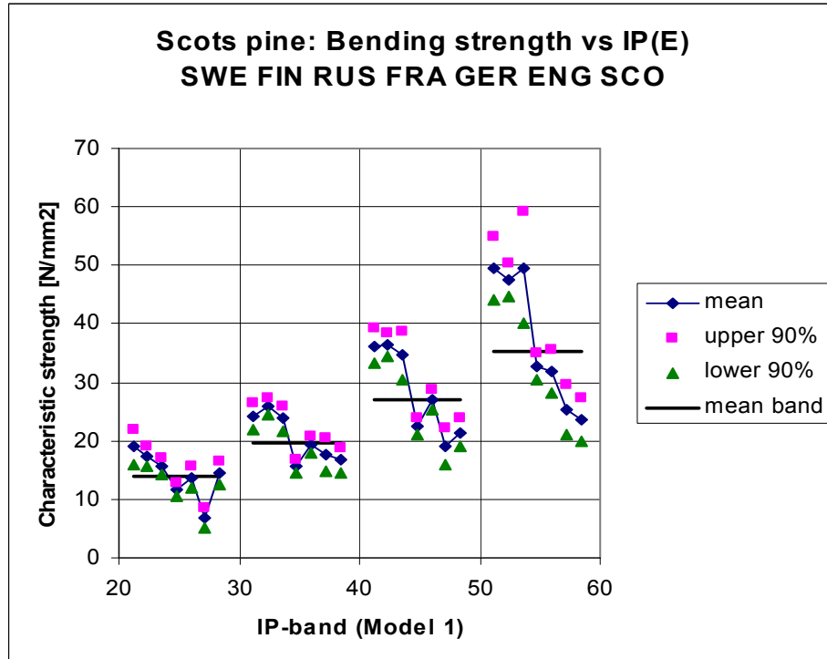
Figure 47. Comparison between countries, characteristic strength values with individual confidence limits. Pine in bending, Model 1.
