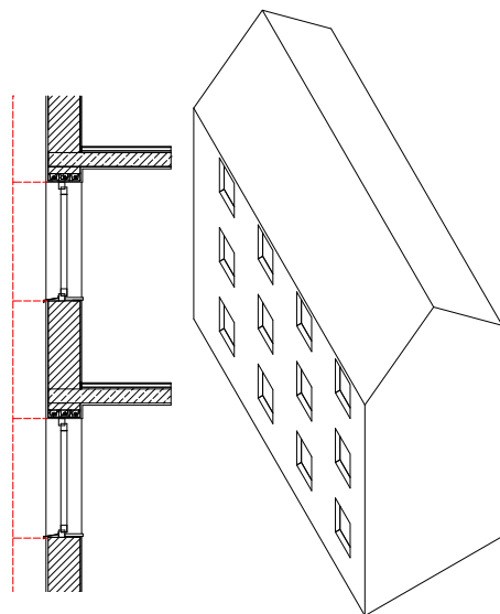
19. Load bearing outer walls versus a skeleton structure with infill.
