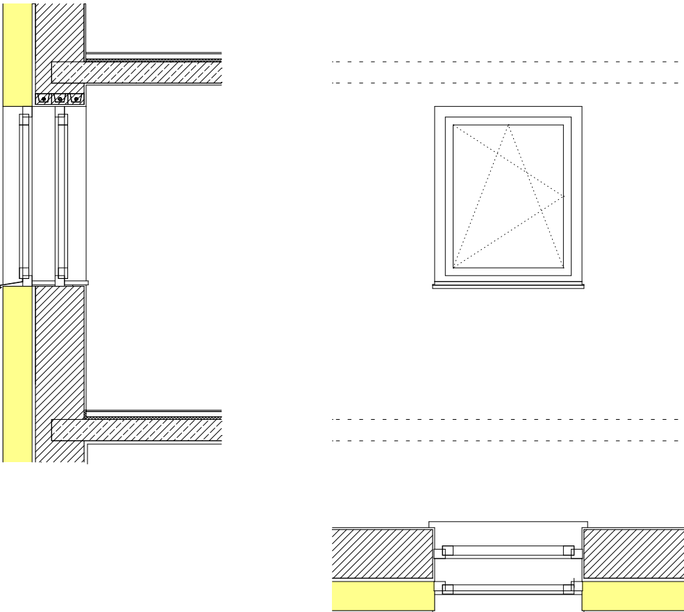
120. Conservation of existing window and an additional exterior window integrated in the insulation layer.
