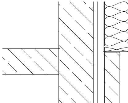
25. Separate foundation
