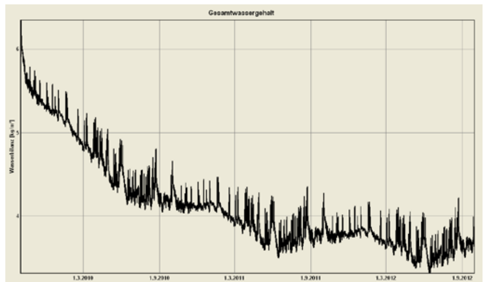
157. Simulation of existing wet wall with 18 cm TES EnergyFaçade done with WUFI® 4.2. The graph shows the decrease of the total amount of water in the entire, insulated exterior wall construction
