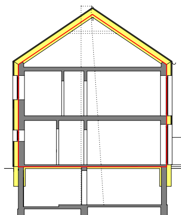
180. Insulated building envelope
