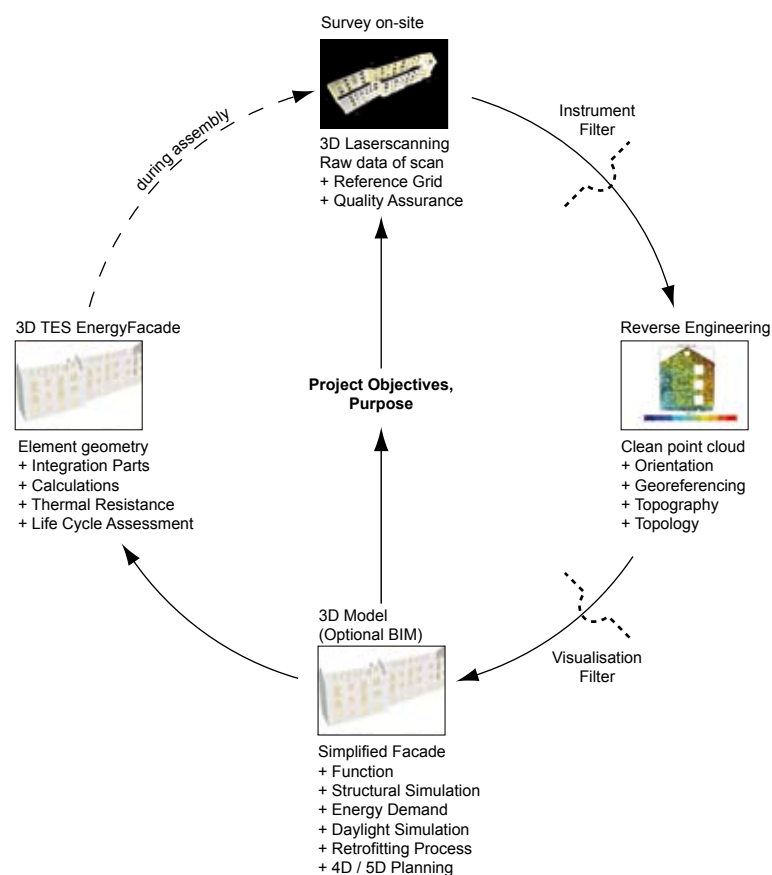
76. Necessary steps of a TES survey campaign based on Scherer's paradigm.
