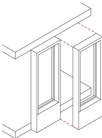
100. Basics concept of an element-façade
