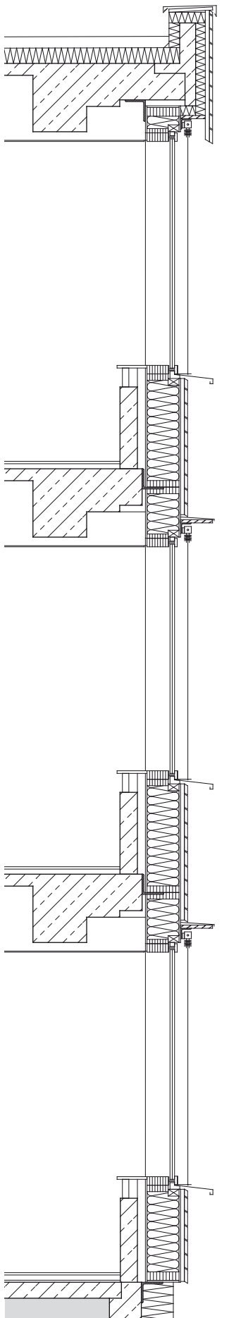
194. CAD/CAM model of elemented façade ready for production.
