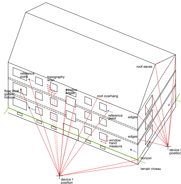
72. Critical points of a façade survey.
