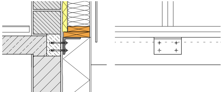
136. L- bracket with a sill beam. Exchange of brick layer in front of the ceiling, grouting closer.
