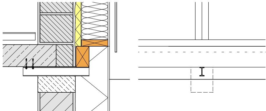
137. Cantilever beam e.g. IPE rocker. Fixation under basement ceiling, grouting closer
