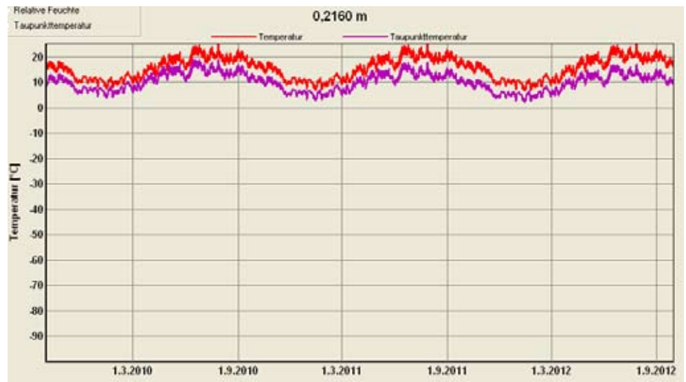
158. Temperature and dew-point diagram of the adaption layer during a range of three years. The red line indicates the temperature curve while the pink line shows the dew point temperature. The position is on the outside of the wood fibre hard board or the interior side of the TES element.
