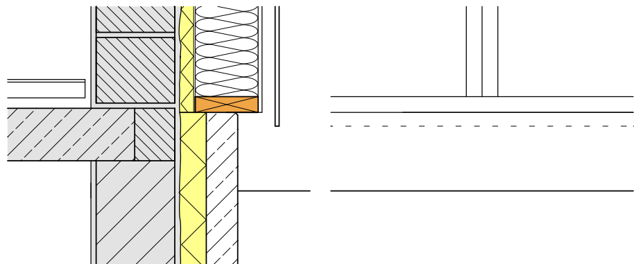
138. Foundation Precast concrete component, frost resistance founded, adaption layer thermal insulation.
